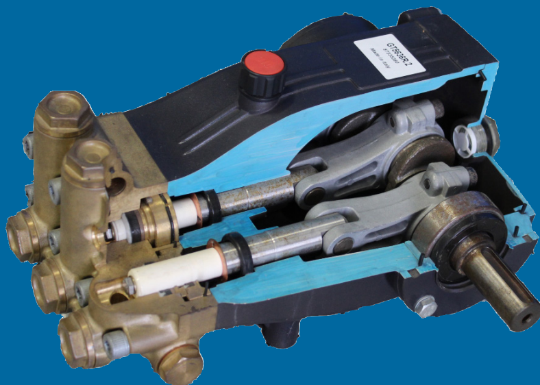
IDENTIFYING CAVITATION DAMAGE IN TRIPLEX PISTON PUMPS Insufficient water supply; damage to the high pressure seals will be noticeable
